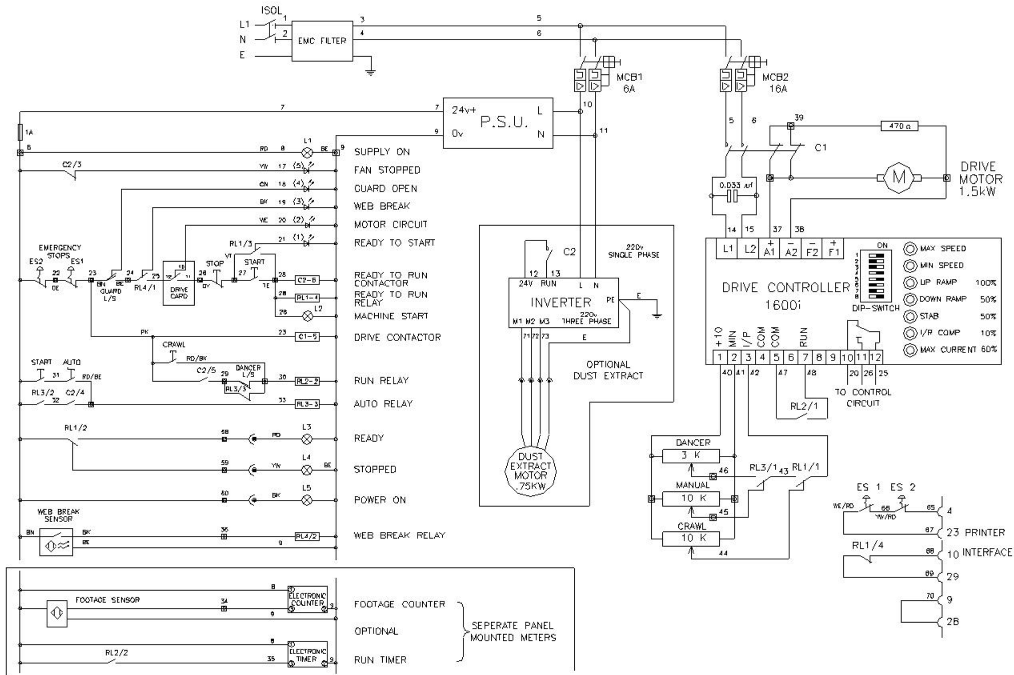
BPP20 CIRCUIT DIAGRAM REF 800417 ISS J
